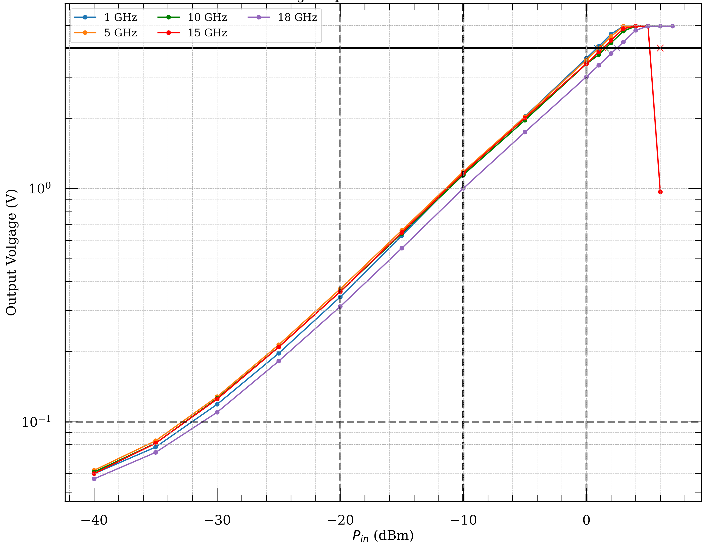
Measured voltage-to-power curve of detector module086
